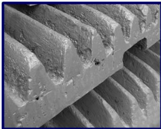
TYPICAL AFTERMARKET JAW PLATE TO SUIT EXTEC C-12
